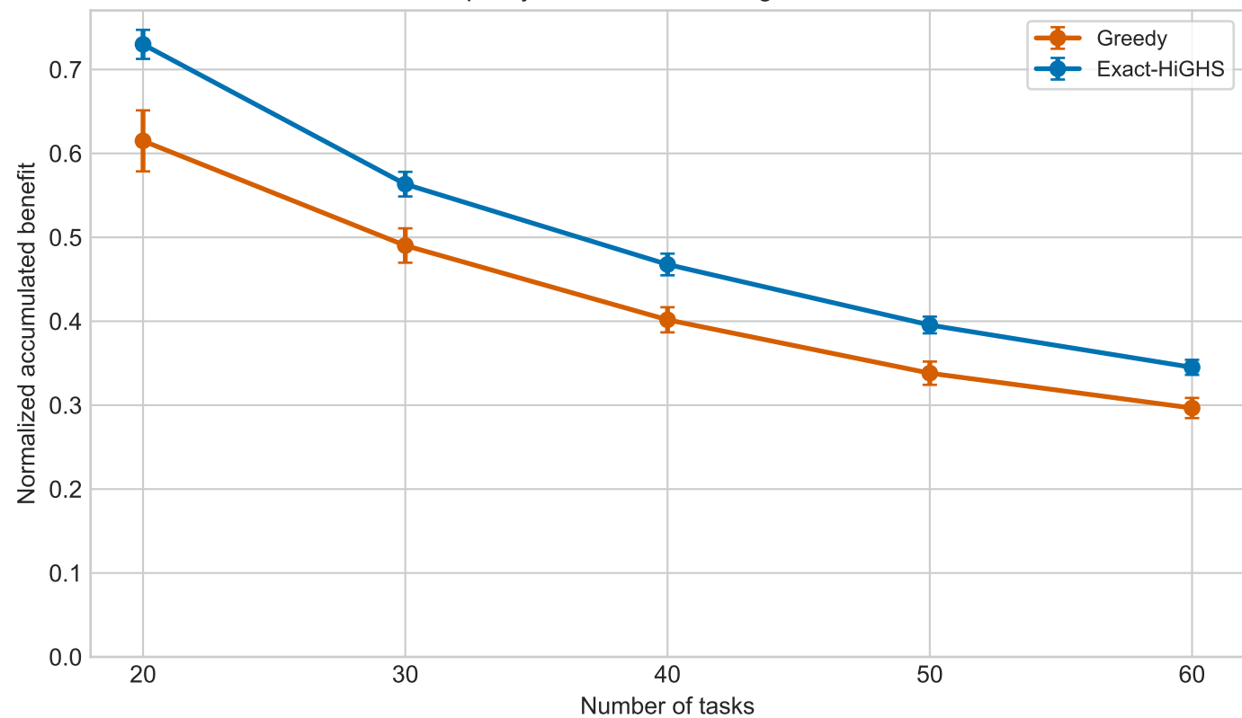
Solution quality with conditional large-instance results
